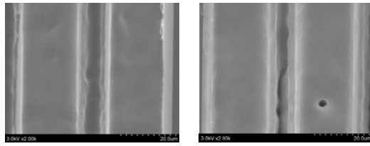
(a) N = 5 shots (b) N = 200 shots (i) \lambda = 355 nm, Q = 1.0 J/cm 2
