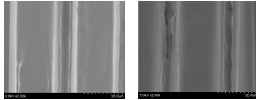
(a) N = 5 shots (b) N = 200 shots (ii) \lambda = 532 nm, Q = 1.0 J/cm 2
