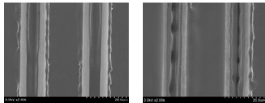
(a) N = 5 shots (b) N = 200 shots (iii) \lambda = 1064 nm, Q = 1.0 J/cm 2
