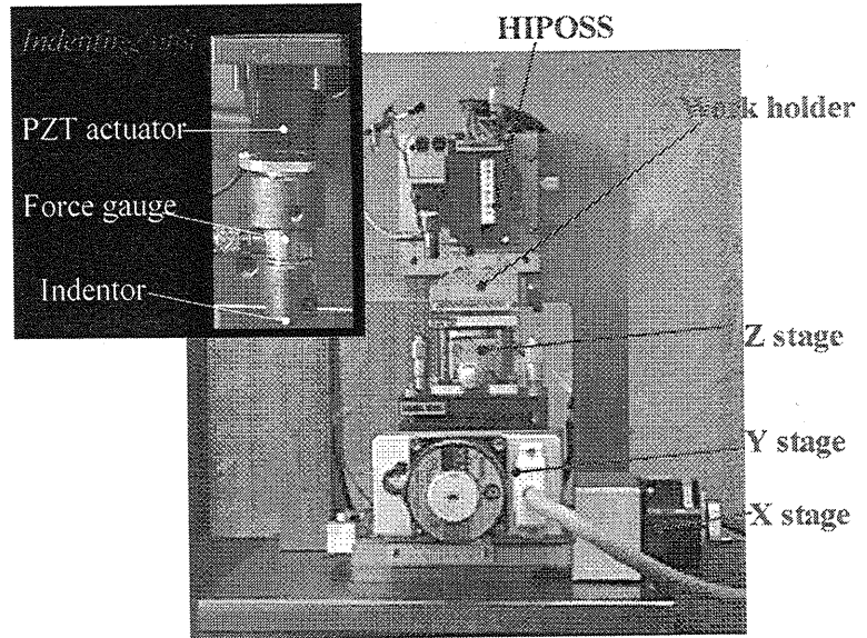
Fig.8 Photograph of multi dimpling machine
