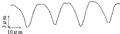
Fig.11 Example of dimple profile
